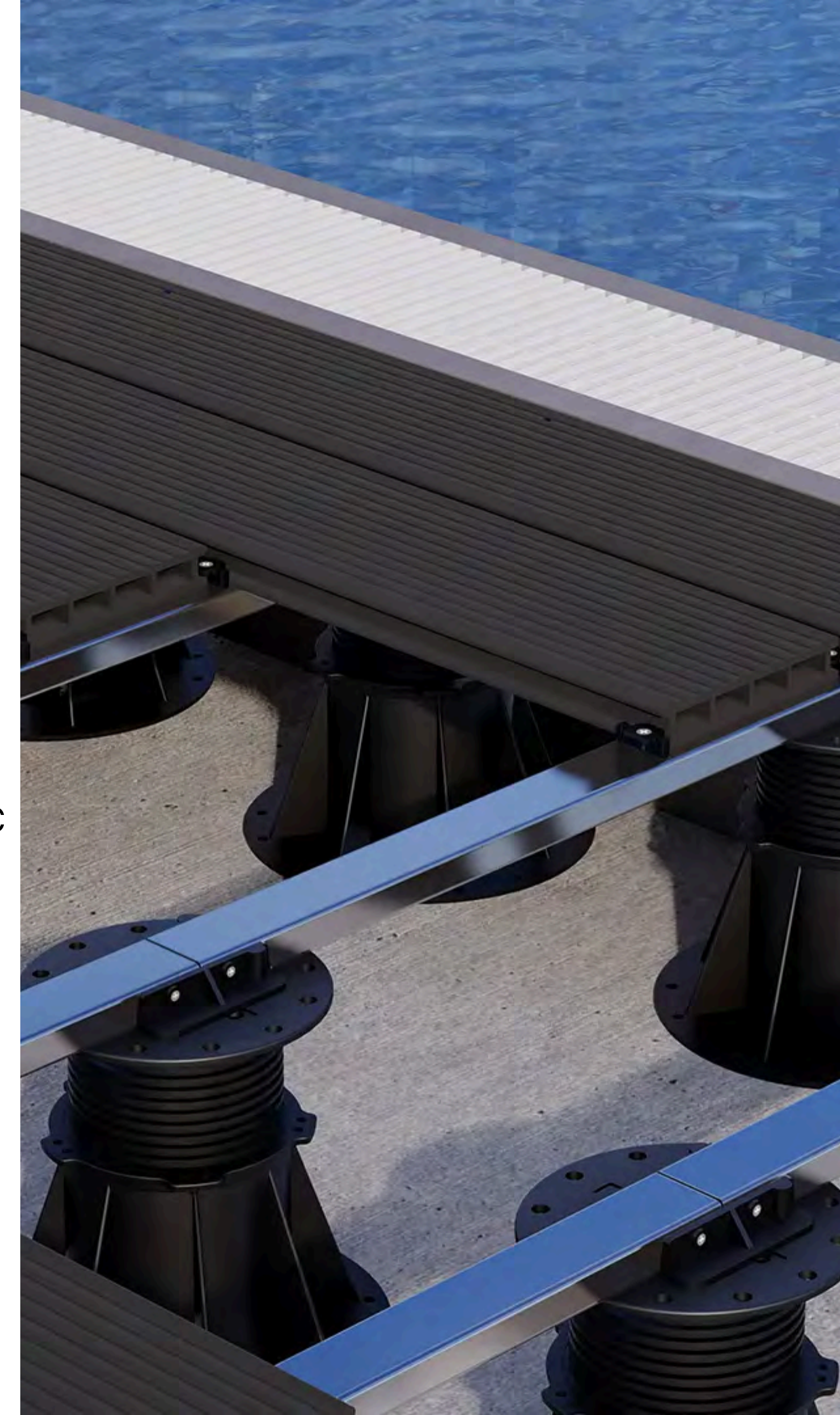
Fixing element
